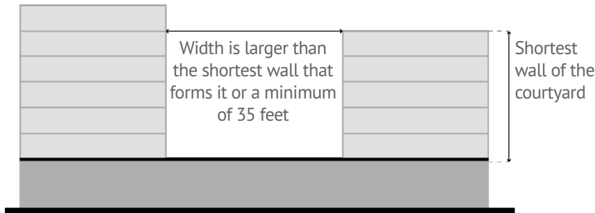
FIGURE 9: ENCLOSED COURTYARDS
