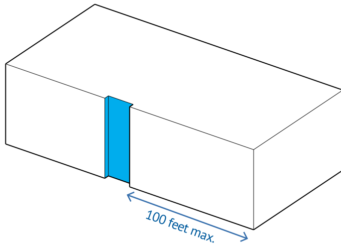
FIGURE 3: MASSING BREAKS
